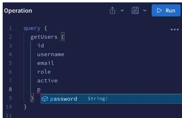
Figure 13.16: Autocomplete
