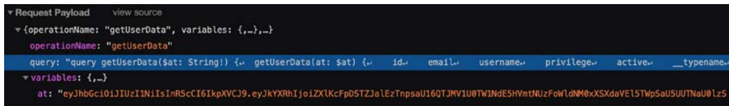
Figure 13.35: getUser data
