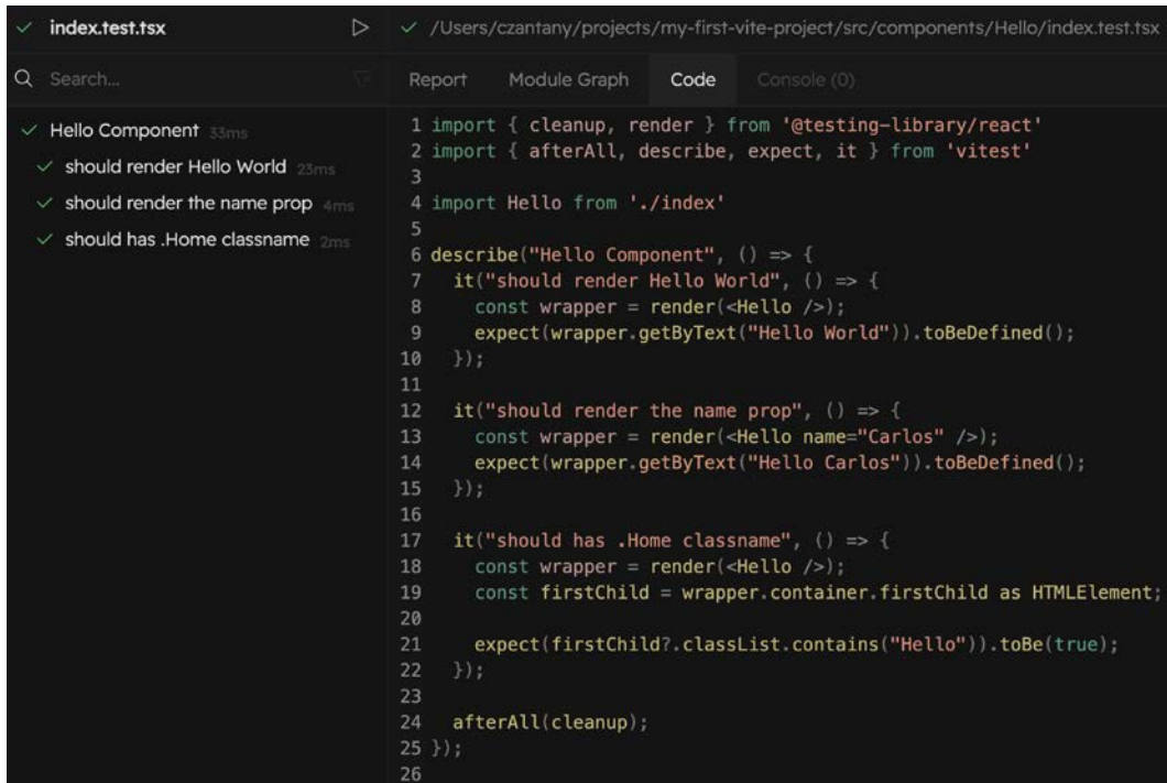
Figure 16.11: Code
