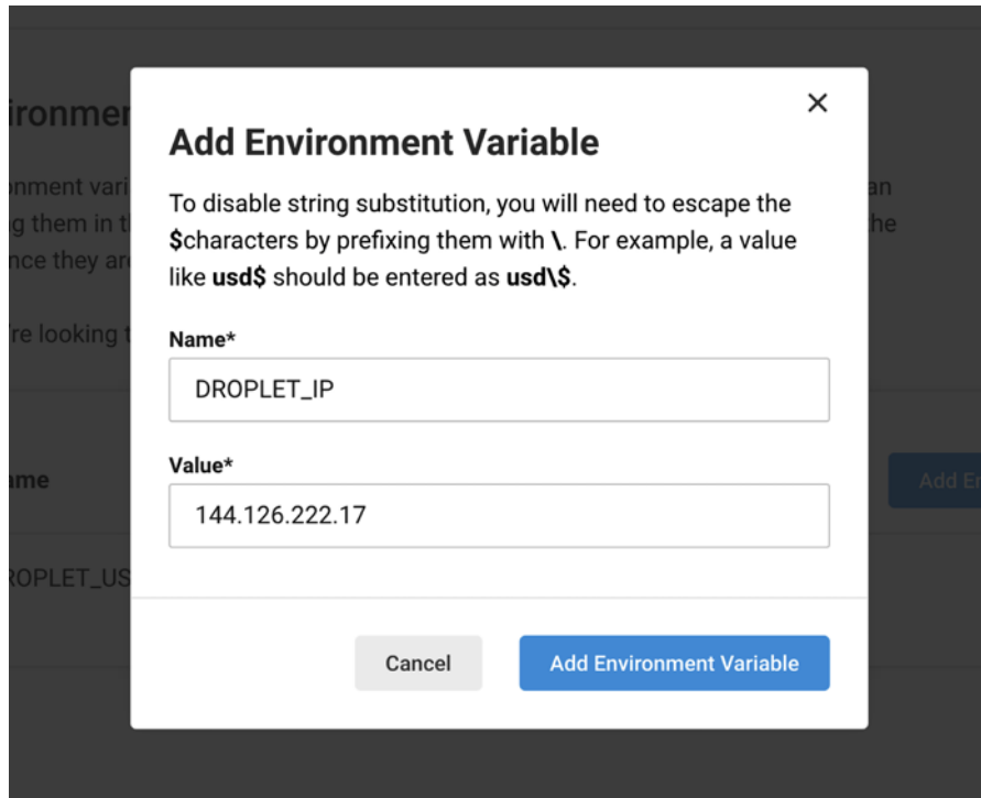
Figure 17.36: DROPLET_IP
