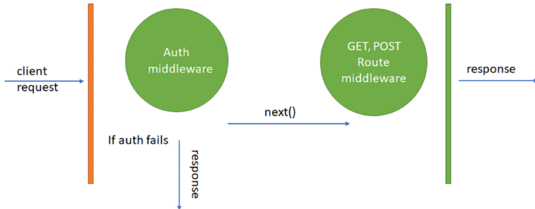
Figure 13.28: Auth middleware
