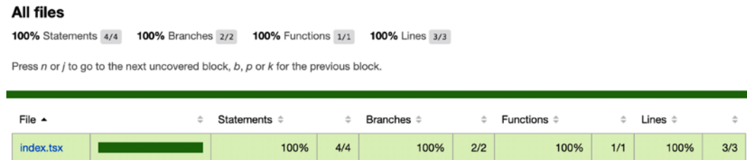
Figure 16.4: Lcov-report
