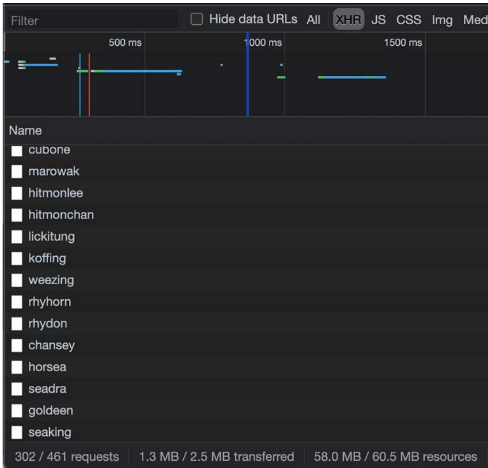
Figure 11.8: 151 requests
