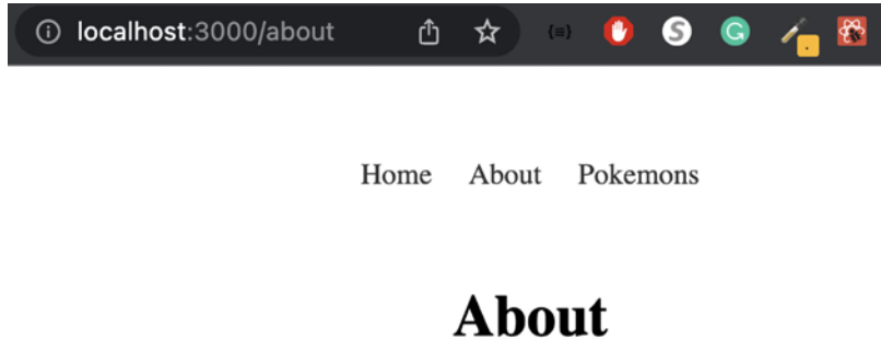
Figure 9.10: About page
