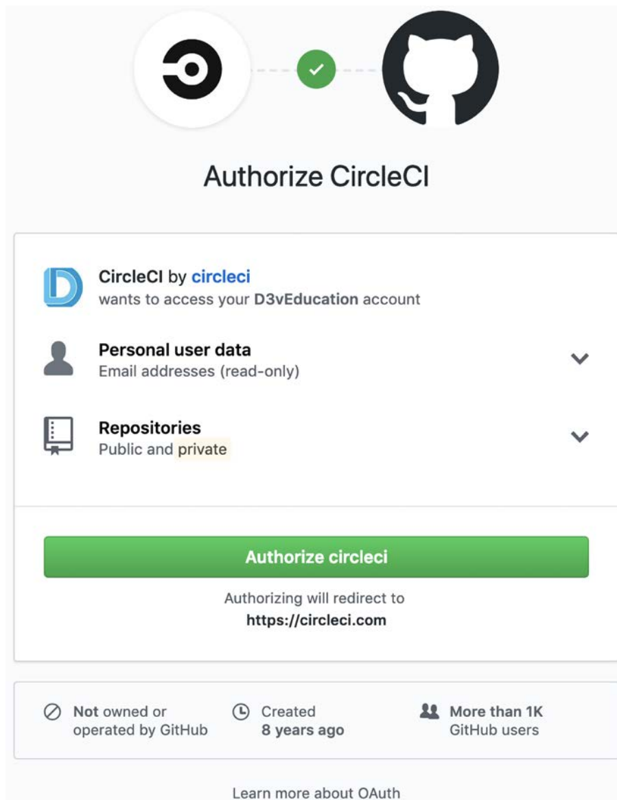
Figure 17.31: Authorize CircleCI
