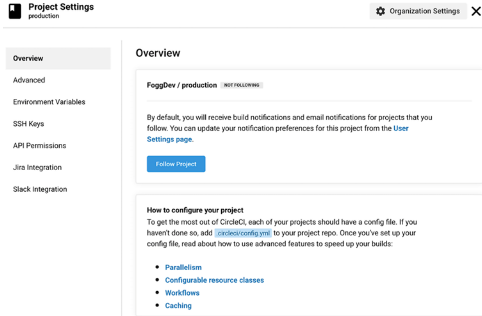
Figure 17.32: Project Settings
