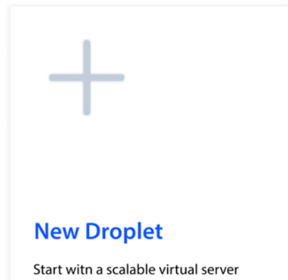
Figure 17.3: New Droplet
