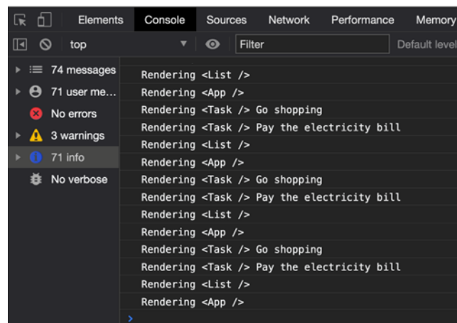
Figure 8.15: Bad performance
