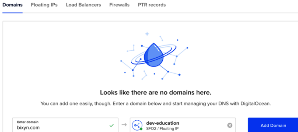
Figure 17.28: Networking
