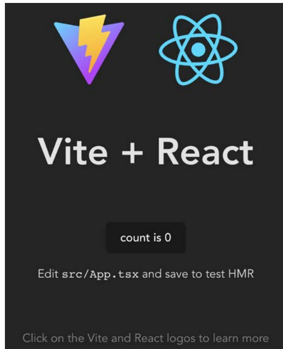
Figure 16.7: Vite app
