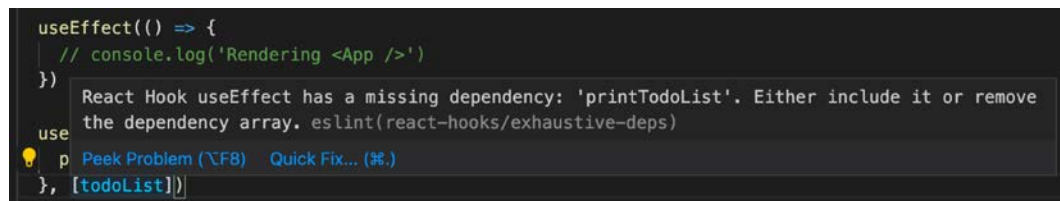
Figure 8.19: react-hooks/exhaustive-deps
