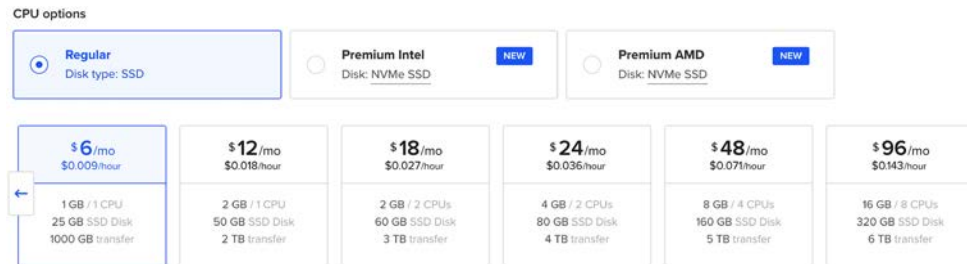
Figure 17.6: CPU options
