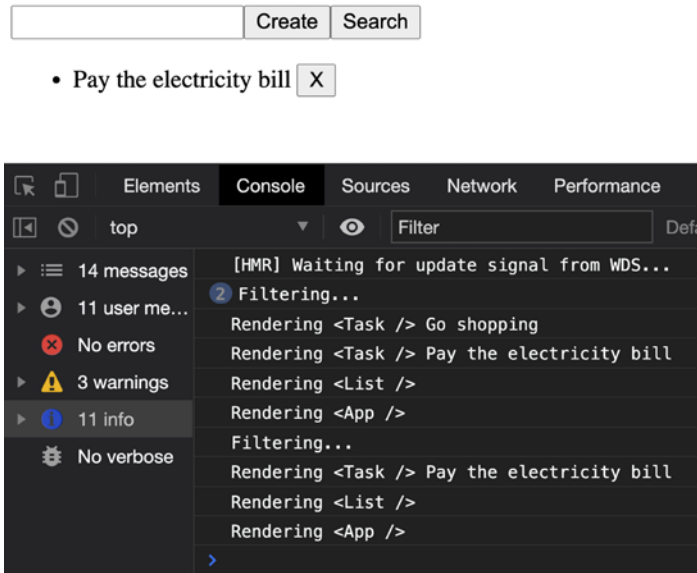
Figure 8.17: Deleting tasks
