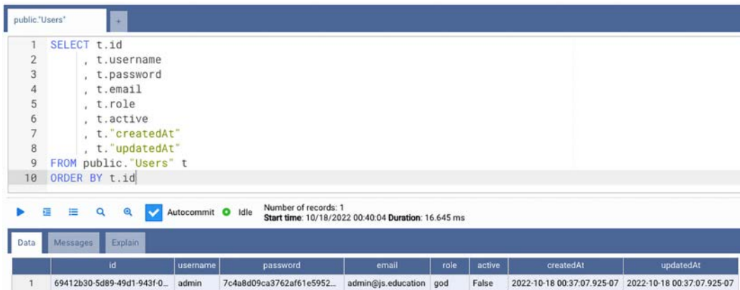
Figure 13.11: Database query
