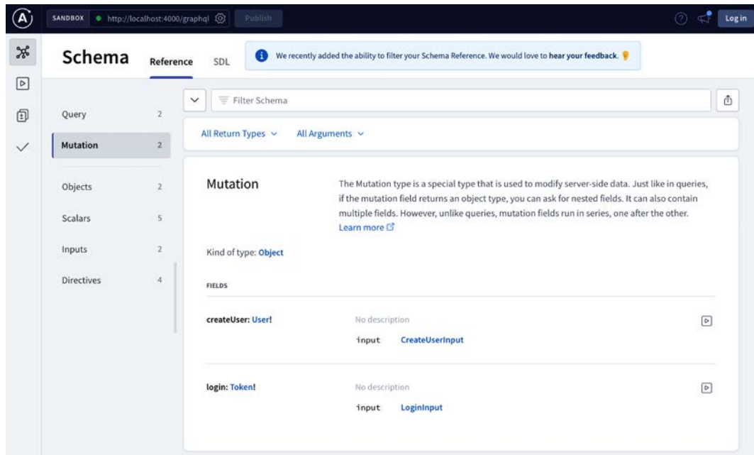
Figure 13.7: Schema
