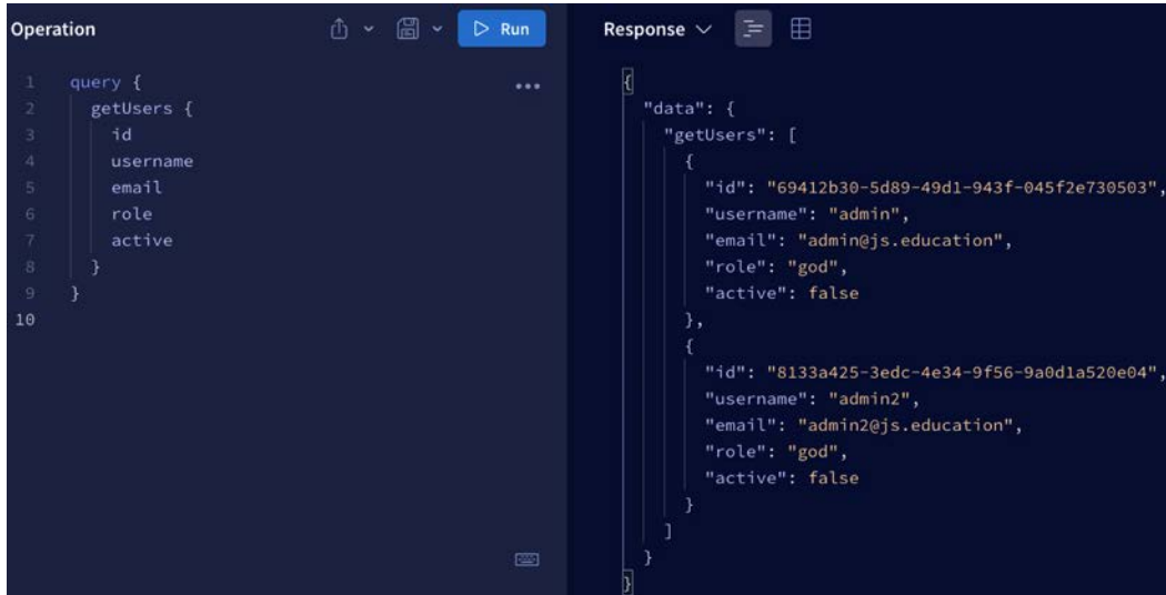
Figure 13.15: getUsers query
