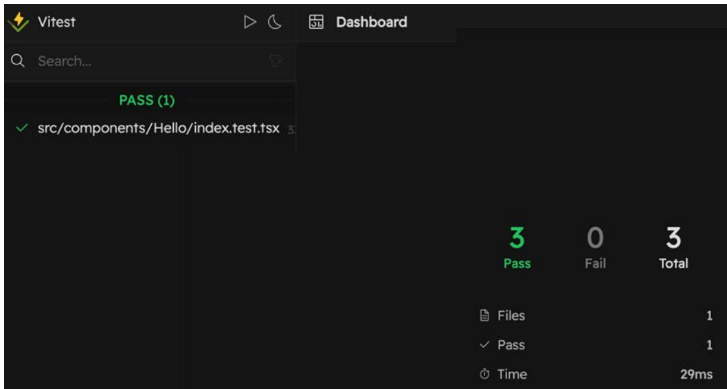
Figure 16.9: Vitest UI
