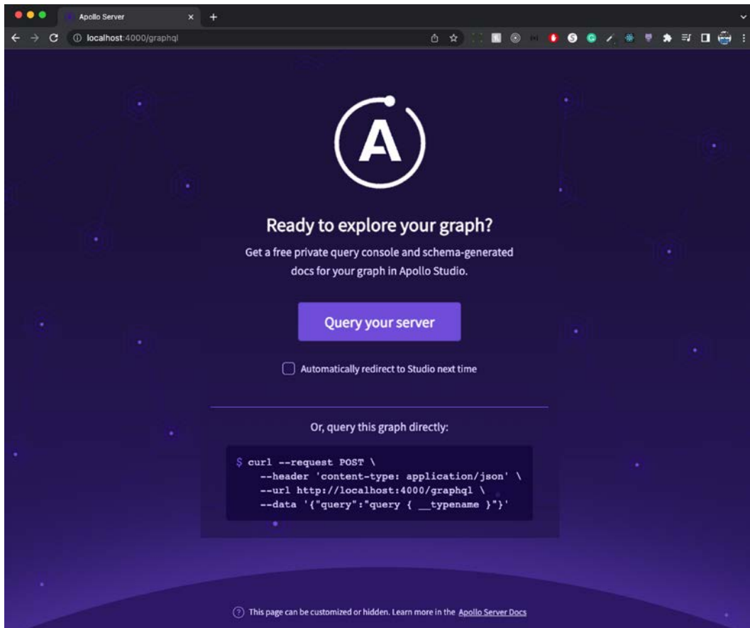
Figure 13.5: GraphQL Explorer
