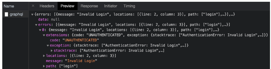
Figure 13.33: Invalid login
