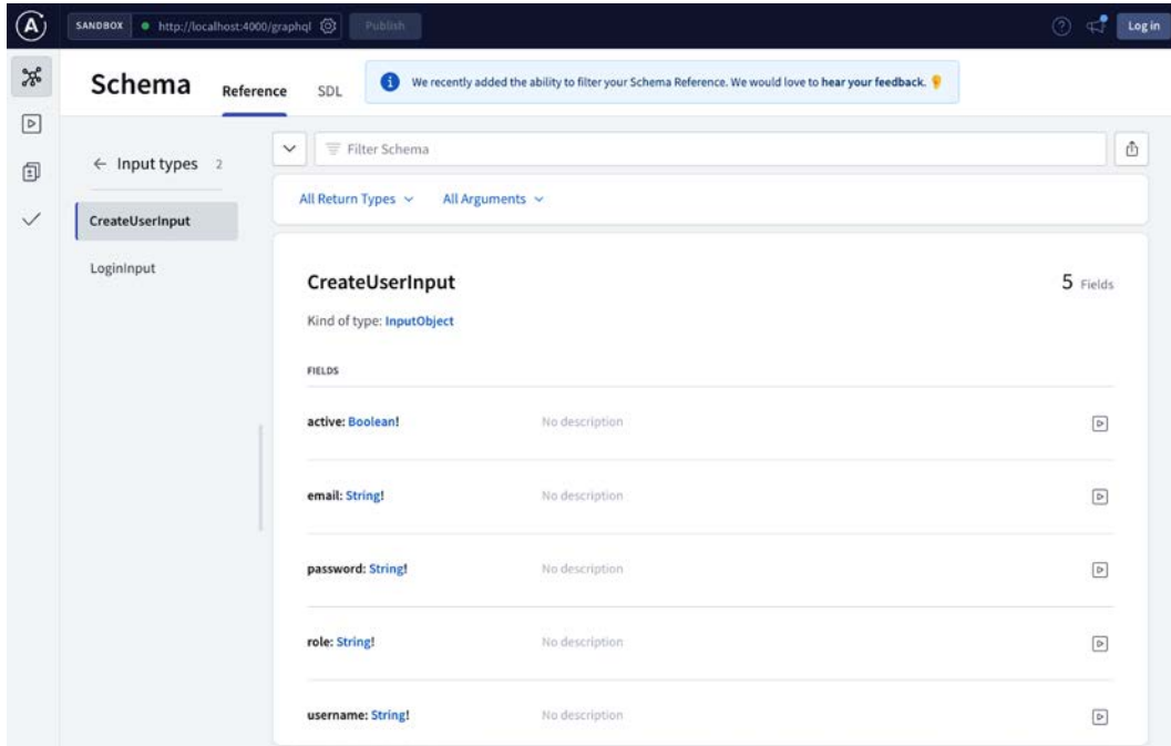
Figure 13.8: CreateUserInput
