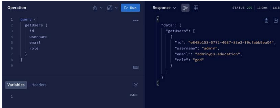
Figure 13.10: getUsers query
