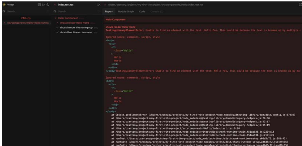
Figure 16.12: Failing test
