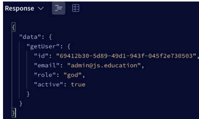
Figure 13.24: getUser data
