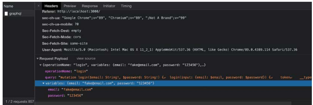
Figure 13.32: GraphQL request
