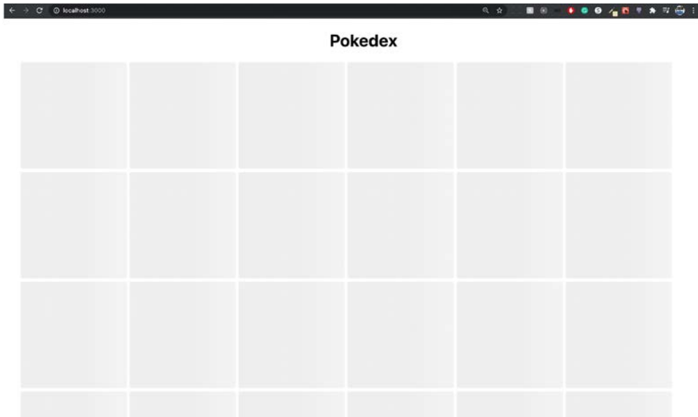
Figure 11.4: SkeletonLoading
