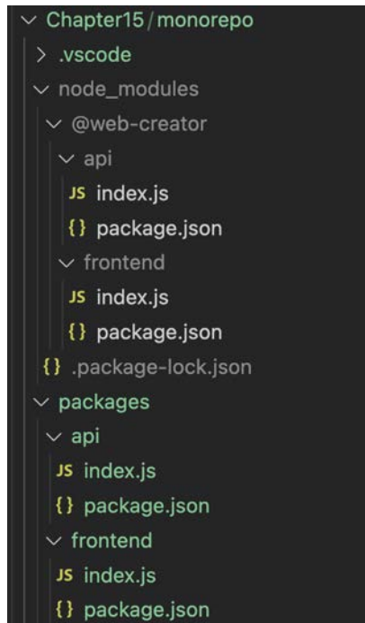
Figure 14.2: Monorepo structure
