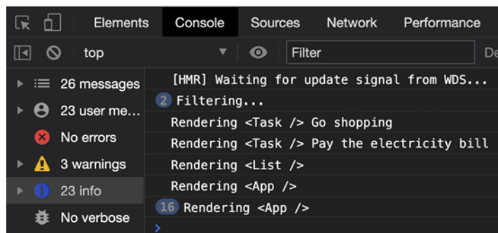
Figure 8.16: Improving performance
