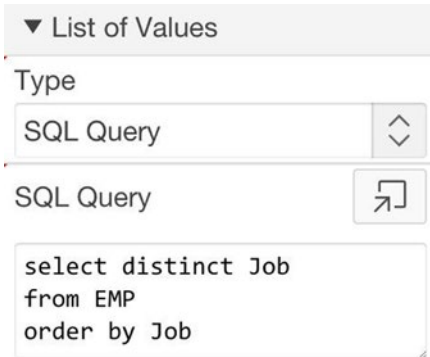
Figure 5-10. Specifying the autocomplete list
